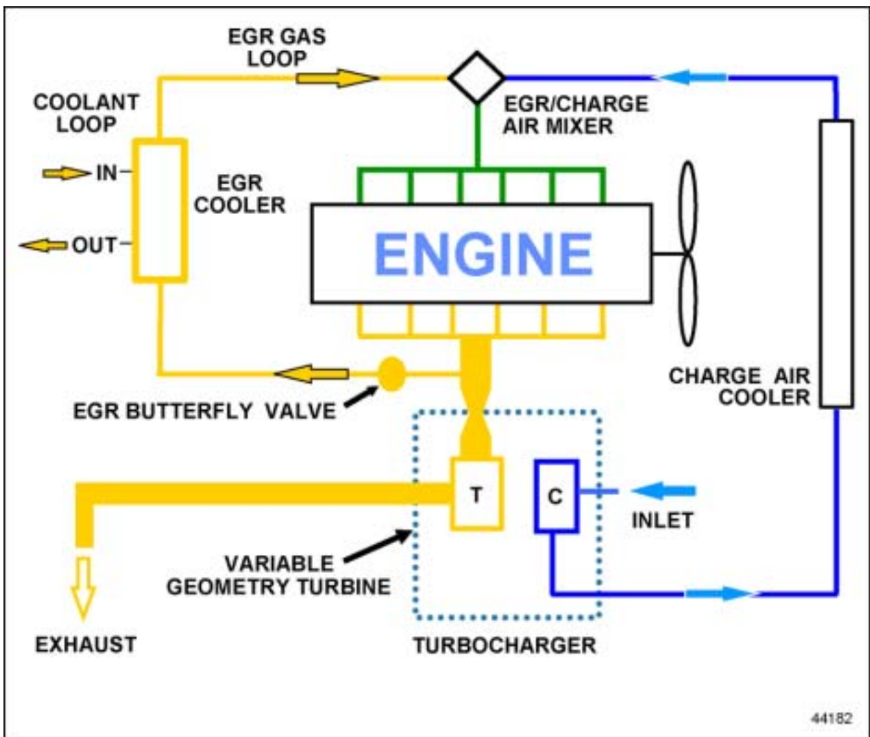
Figure 2-1 EGR System
